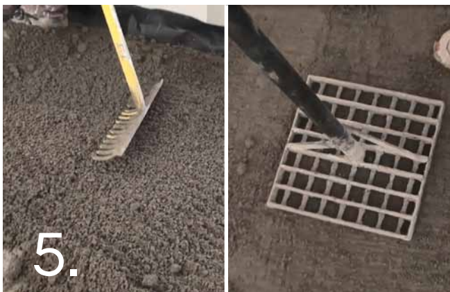
5. Spread screed mix evenly and compact. Do not compact screed that is too thick in one go. Compact in multiple stages depending on the thickness of the screed.
